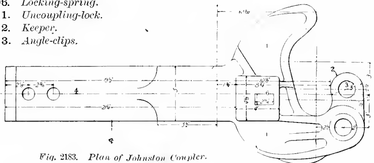
Fig. 2183. Plan of Johnston Coupler.
